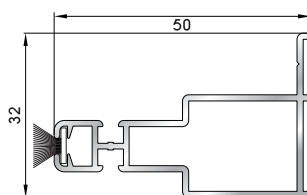
094400 Opposite profile with woven weatherstripping pile for one leaf horizontal movement insect screen (4,5m)
