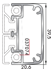
"T" profile for opening-out insect screen (6m)
