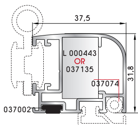
Leaf for opening-out insect screen (6,3m)
