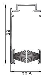
094401 Opposite profile with magnet for one leaf horizontal movement insect screen (4,5m)
