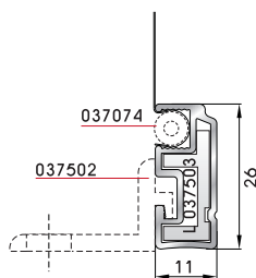
Fixed insect screen profile for frame and "T" profile (6m)
