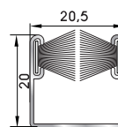
096305 Insect screen low guide with woven weatherstripping pile and double face self-adhesive tape (6m)
