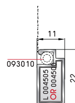
Fixed insect screen profile for frame and "T" profile (6m)
