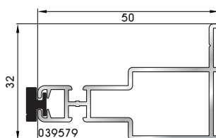
094401 Opposite profile with magnet for one leaf horizontal movement insect screen (4,5m)
