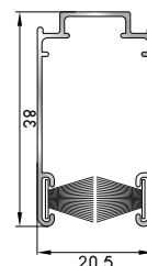
094400 Opposite profile with woven weatherstripping pile for one leaf horizontal movement insect screen (4,5m)
