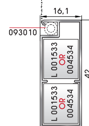
Fixed insect screen profile for frame and "T" profile (6m)
