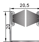
096305 Insect screen low guide with woven weatherstripping pile and double face self-adhesive tape (6m)
