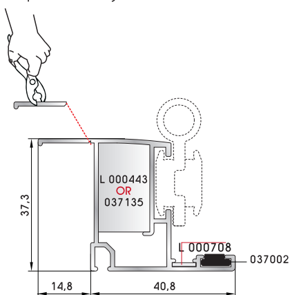
Frame for opening-out insect screen (5,5m)
