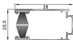
096302 Insect screen guide with woven weatherstripping pile (6m)
