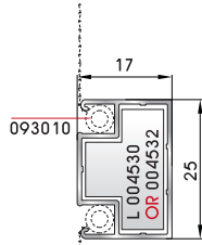
Fixed insect screen profile for frame and "T" profile (6m)
