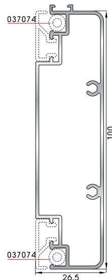
Muntin for opening-out insect screen (6m)
