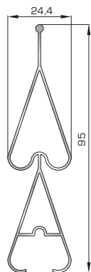
40475 W=59.1\text{gr/m} A=0.306\text{m}^2/\text{m}
