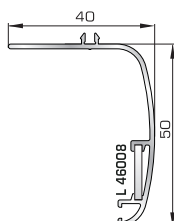
Round screwing casing trim 50mm
