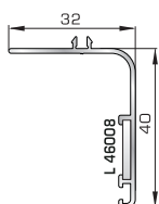
Flat screwing casing trim 40mm
