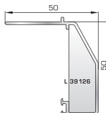
Canted screwing casing trim 50mm
