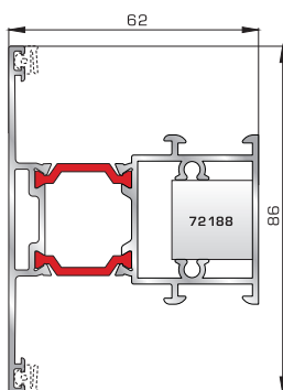
Sash muntin 62mm (for 70615, 70665 70895, 70875 sash profiles)
