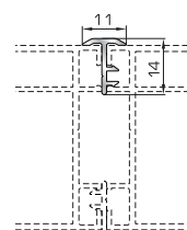
Hooked casing trim for frame coupling
