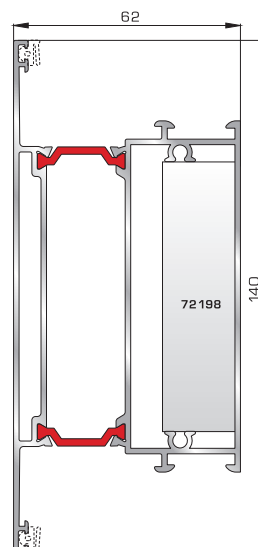
Sash muntin 62mm (Big) (for 70615, 70665 70895, 70875 sash profiles)
